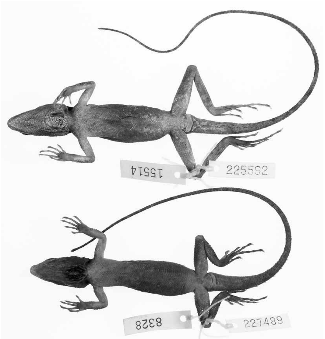
FIGURE 7. Ventral view of the holotype of Ptyctolaemus collicristatus , sp. nov., CAS 227489, and P. gularis , CAS 225592. Photographed by Dong Lin.
