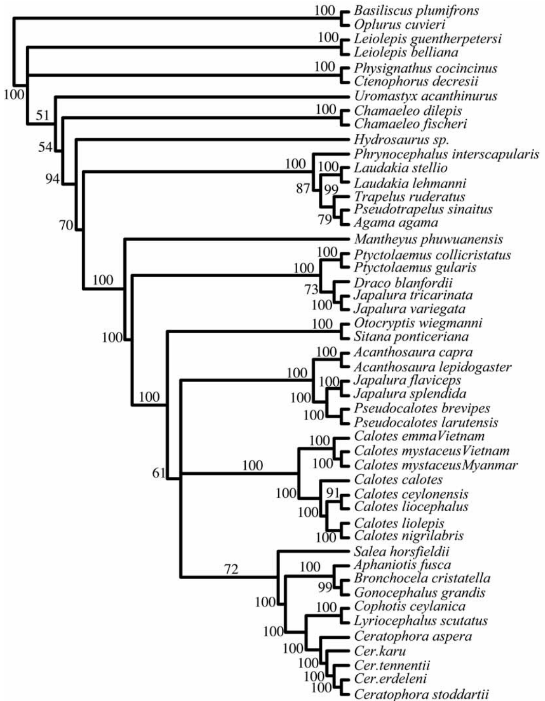
FIGURE 2. Phylogenetic relationships among agamid lizards based on Bayesian analysis using GTR + I + G model (mean -\log -likelihood = 36362.88; variance = 58.95). Tree is a 50% majority rule consensus tree of 200,000 Bayesian trees. Numbers adjacent to branches are percentages of trees recovered with a particular node and represent posterior probability values.
