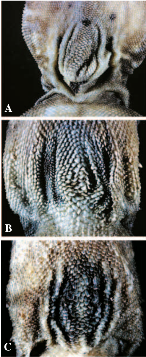
FIGURE 4. View of gular region of (A) P. phuwuanensis , FMNH (HKV 64903); (B) P. gularis , CAS 225592; and (C) P. collicristatus sp. nov., CAS 227489.
