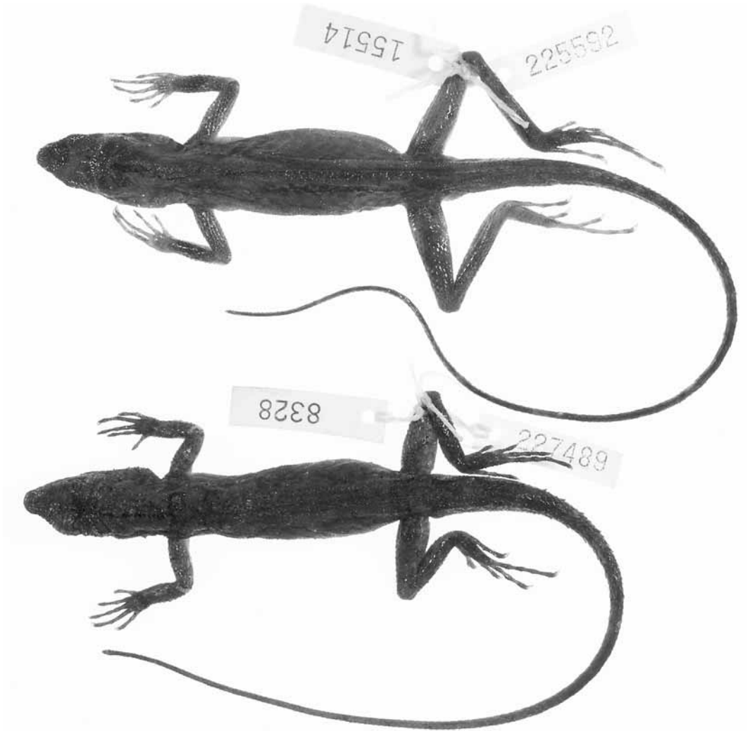
FIGURE 6. Dorsal view of the holotype of Ptyctolaemus collicristatus , sp. nov., CAS 227489, and P. gularis , CAS 225592. Photographed by Dong Lin.
