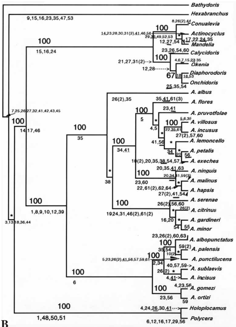
branches are the percentage of the 3 consensus trees that agree on this node. The asterisk also denotes 100% agreement on the node. Numbers shown at the branches are character numbers from Table 2. The underlined numbers indicate reversals.
