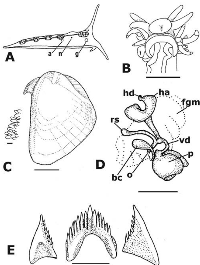
FIGURE 5. Flabellina dana sp. nov. (St. Lucia). A. Right lateral view showing position of ceratal insertions. Key: a, anus; n, nephroproct; g, genital apertures. B. Ventral view of head and foot. Scale bar = 1 mm. C. One jaw plate, scale bar = 200 \mu m and masticatory margin enlarged to show denticles, scale bar = 10 \mu m. D. Reproductive system drawn using a camera lucida. Scale bar = 0.5 mm. Key: bc, bursa copulatrix; fgm, female gland mass; ha, hermaphroditic ampulla; hd, hermaphroditic duct; o, oviduct; p, penis; rs, receptaculum seminis; vd, vas deferens. E. One row of radular teeth. Scale bar = 25 \mu m.
