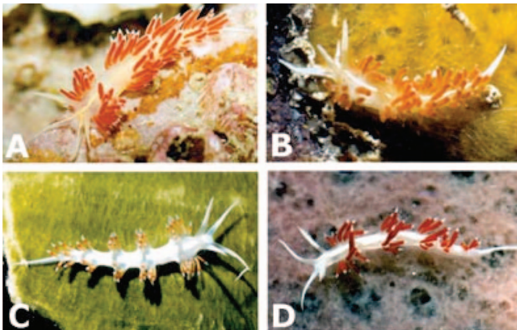
FIGURE 1. Living animals. A. Flabellina verta with yellow lines, Testigos, Venezuela B. Flabellina verta with white lines, Miami, Florida. C. Flabellina dushia , Martinique D. Flabellina dana sp. nov., St. Lucia. All photos by Jeff Hamann.
