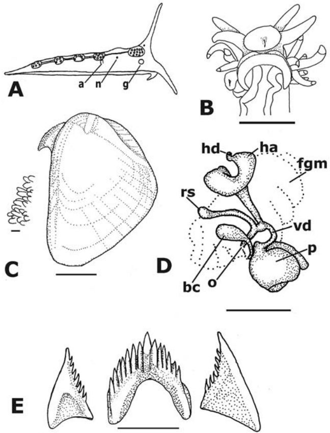
FIGURE 3. Flabellina verta (Sarasota, Florida). A. Right lateral view showing position of ceratal insertions. Key: a, anus; n, nephroproct; g, genital apertures. B. Ventral view of head and foot. Scale bar = 1 mm. C. One jaw plate, scale bar = 200 \mu m and masticatory margin enlarged to show denticles, scale bar = 10 \mu m. D. Reproductive system drawn using a camera lucida. Scale bar = 0.5 mm. Key: bc, bursa copulatrix; fgm, female gland mass; ha, hermaphroditic ampulla; hd, hermaphroditic duct; o, oviduct; p, penis; rs, receptaculum seminis; vd, vas deferens. E. One row of radular teeth. Scale bar = 25 \mu m.
